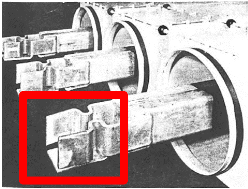
Figure 1 - Plating of Conductor Stab
