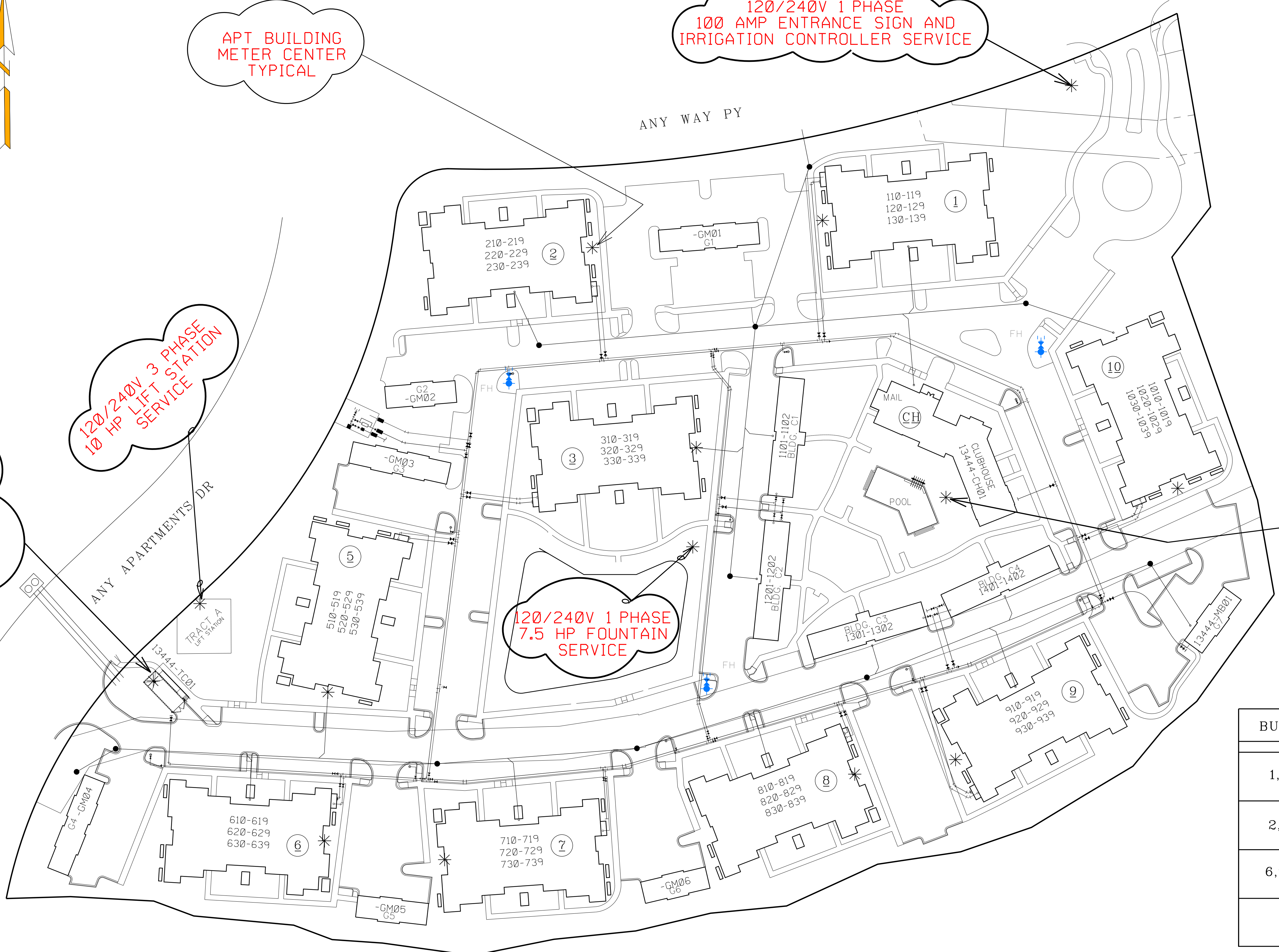
APARTMENT ELECTRICAL MASTER SITE PLAN
