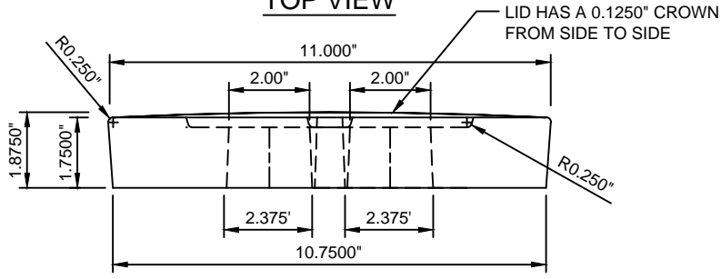
END PROFILE
