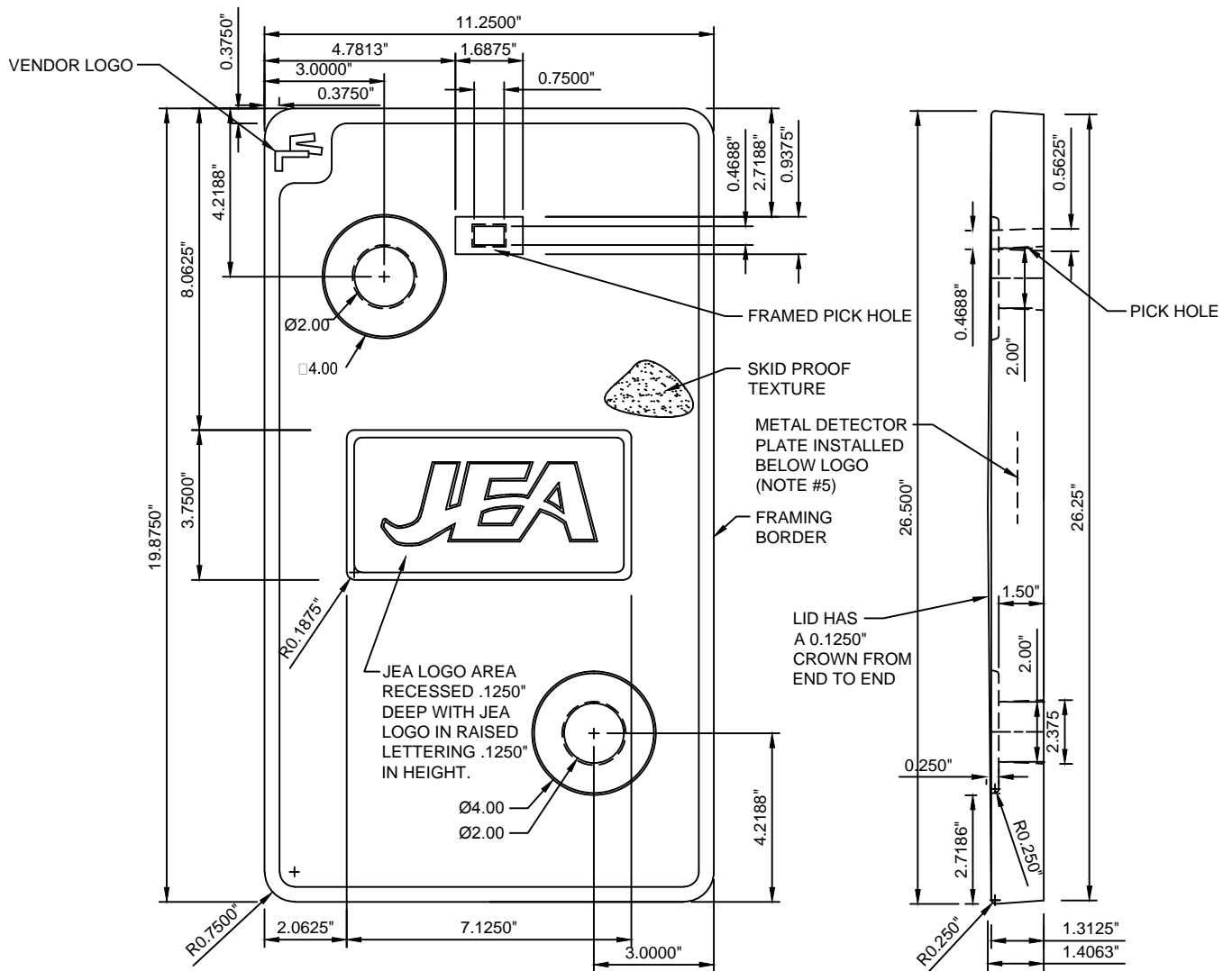
TOP VIEW
