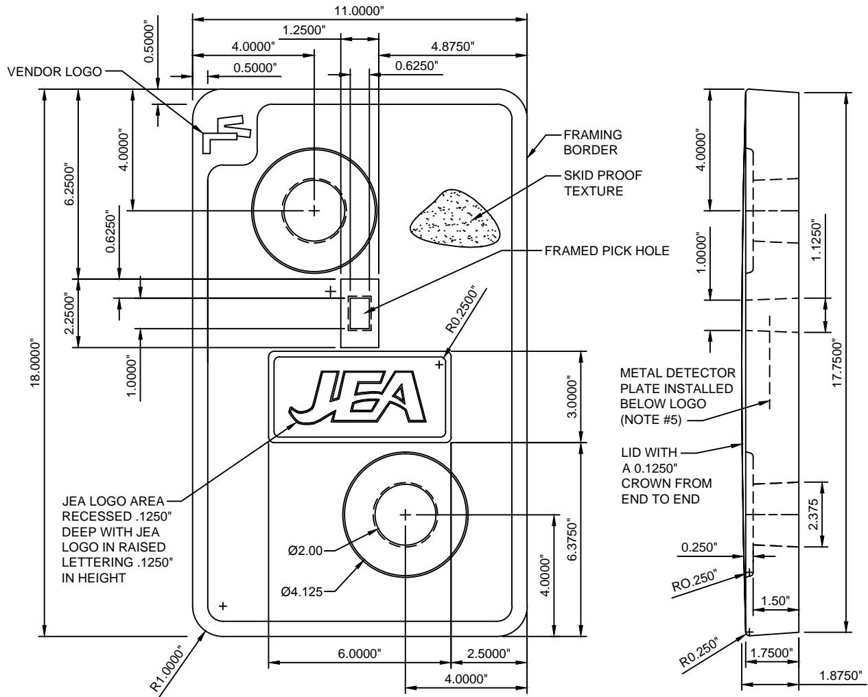
TOP VIEW
